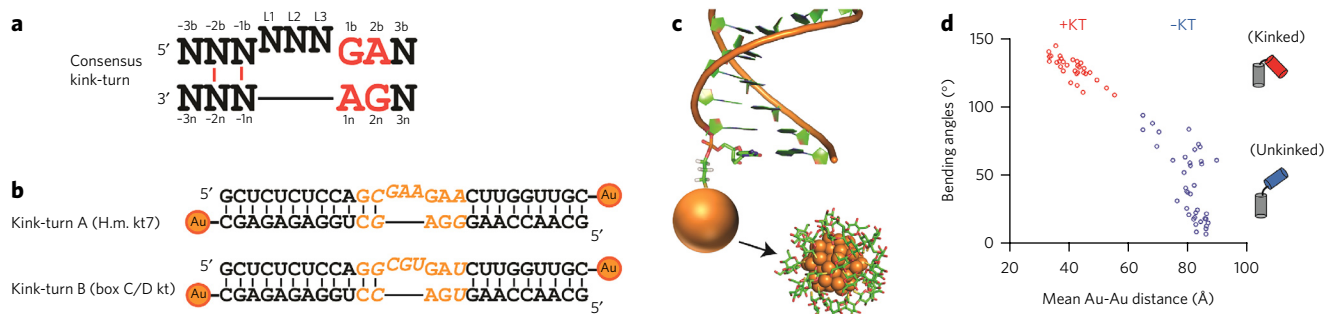
Figure 1 | RNA kink-turns and Au-conjugated constructs. (a) The consensus kink-turn sequence. The -1 and -2 positions are usually canonical base pairs (red lines) 19,23 . (b) Kink-turn sequences investigated in this study. Kink-turn A (KtA) and kink-turn B (KtB) are also known as H.m. Kt7 and box C/D kt, respectively. For simplicity, they are referred to as KtA and KtB in this article. Au nanocrystals were attached to the 3' ends of each strand. The varied kink-turn motif regions are shown in orange; the flanking sequences are the same for the two constructs. (c) Illustration of an RNA helix labeled with a Au nanocrystal (orange sphere) at its 3' end through a three-carbon thiol linker (3'-thiol-modifier C3, Glen Research). A full representation of the nanocrystals (indicated by arrow), including the thioglucose shell, is reproduced from Figure 2c of ref. 18 and was generated on the basis of a substructure of the nanocrystal reported in ref. 48 and the experimental analysis of ref. 49. (d) The distribution of interhelical bending angles and the expected mean Au-Au distance for 70 crystal structures of 0–3 two-way junctions (i.e., 3-nt bulges) with (red) and without (blue) a kink-turn-type 5'-flanking sequence: GA/AN (80% are GA/AG). See Online Methods for a detailed description of how these representative structures were selected and how the expected Au-Au distances were calculated.
